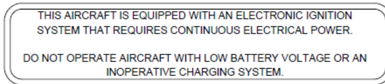
Figure 1: 11-1264 Placard
