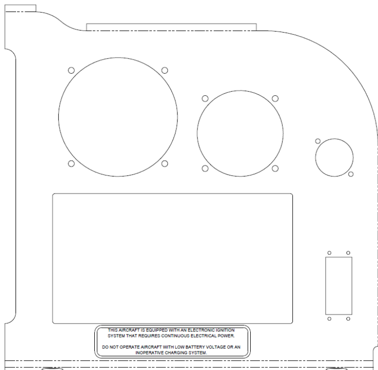
Figure 2: 11-1264 Placard Placement
